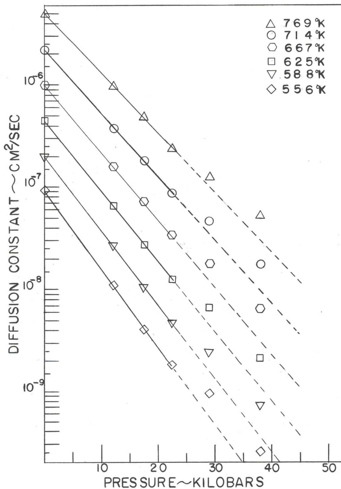
Figure 11. Plot of The Diffusion Constant as a Function of Pressure--Plotted in Isotherms
